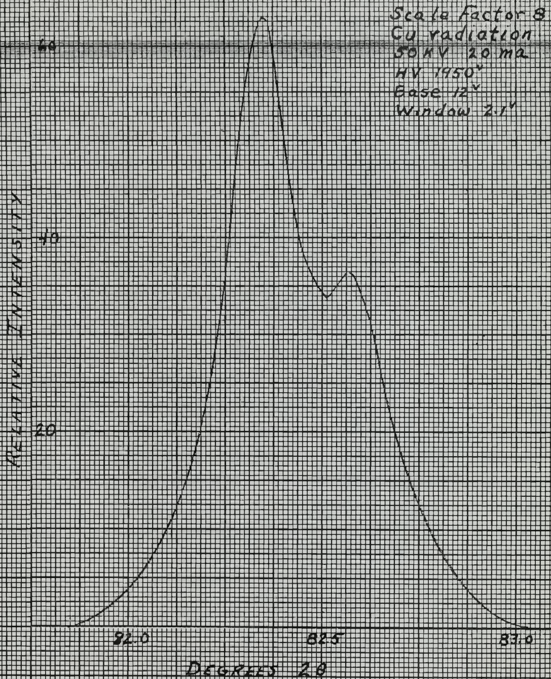
Figure 7 (112) Peak Ductile Specimen
